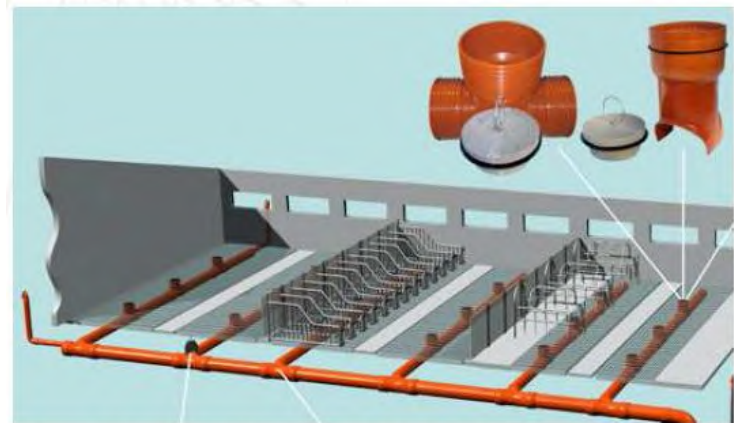
Principle of an indoor slurry system (Straight flush system).
