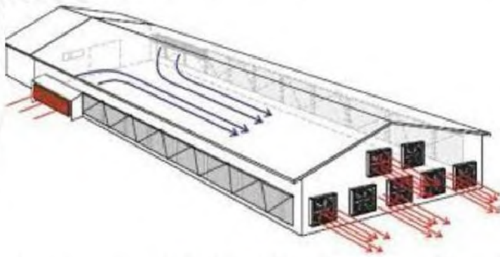
Principle of air Tunnel ventilation system, with cooling pads and gable exhaust fans.
